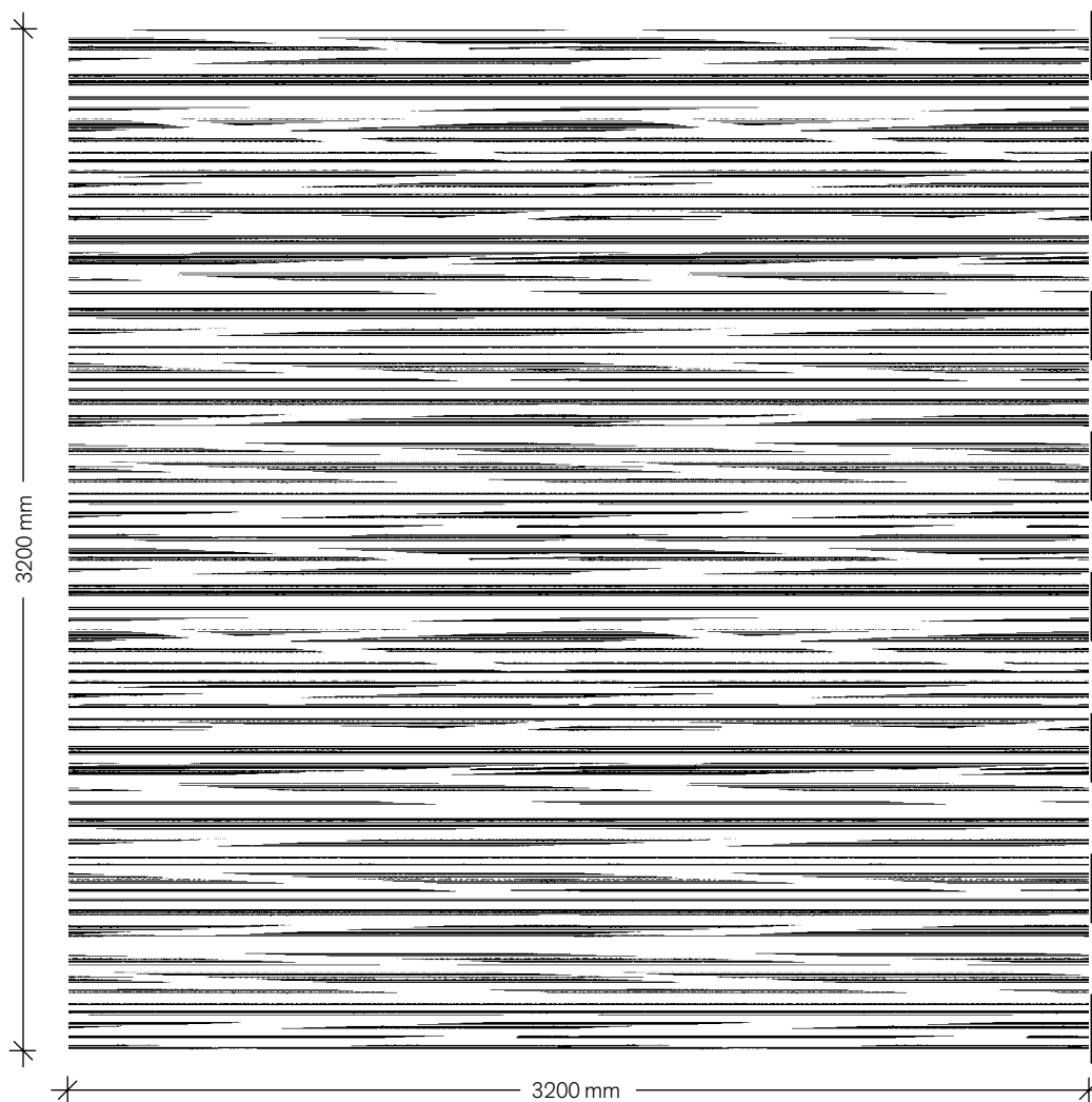
Pattern illustration 1:25
